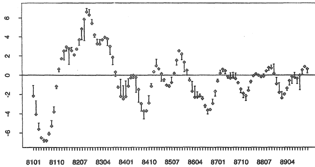
Figure 8. Three-Month-Lagged (-) and Most Recent (◆) Estimates of Percent Changes from the Previous Month in the Trend. Comparison with Figure 7(b) shows that the trend-change estimates calculated three months after the concurrent estimates have much smaller revisions than the latter and fewer changes of sign after revision.
