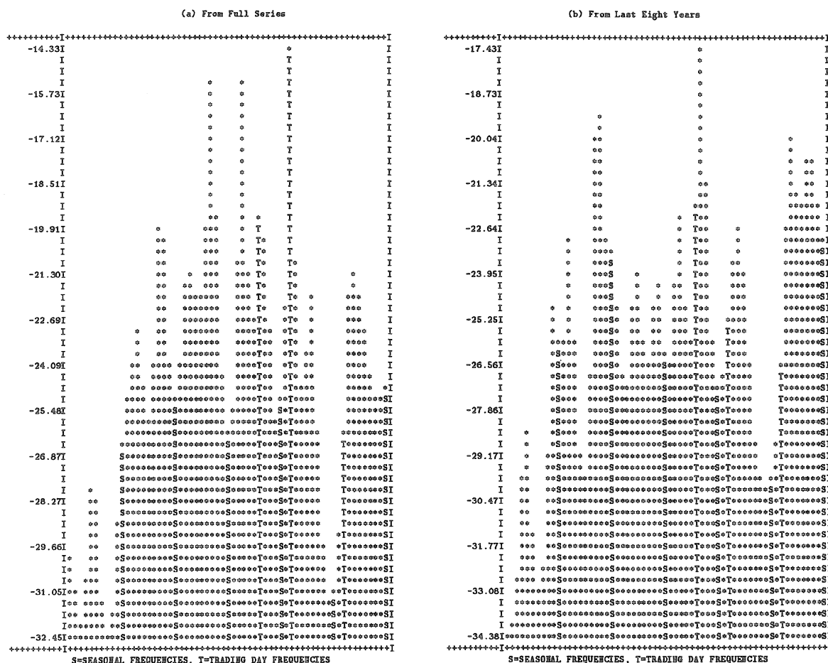
Figure 5. Graphs of the AR Spectrum (7) of the Irregulars of North Central Housing Starts From (a) the Full Series and (b) Its Last Eight Years. The dominant peak at the second trading-day frequency in (a) does not appear in (b). Hypothesis testing confirms the lack of a significant trading-day effect in the last eight years.
